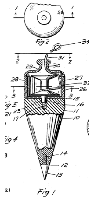
C. G. BYNUM ADJUSTABLE PLUMB BOB Filed Jan. 10, 1948
